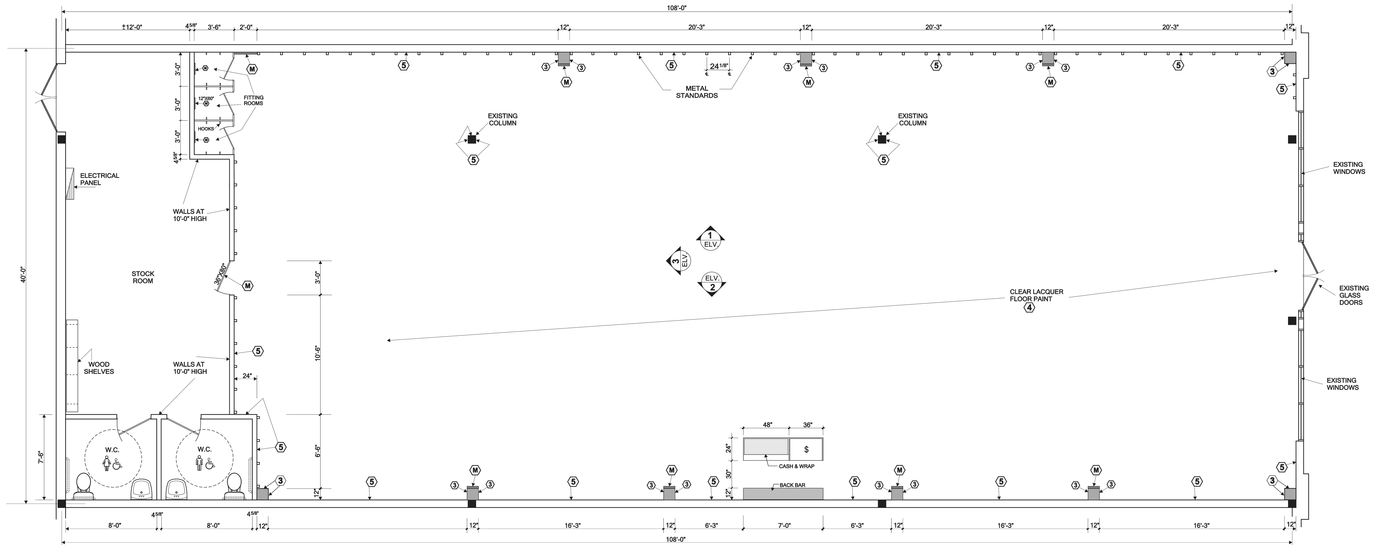
PLAN 1/4" = 1'-0"
