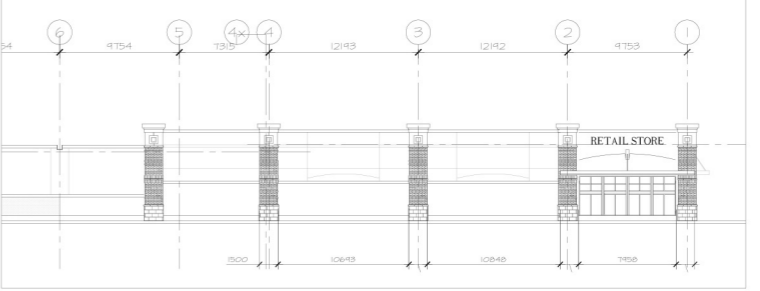
01 FLOOR PLAN A100 1:200
